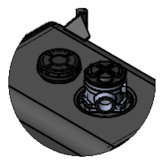
DETAIL B RETURN FILTER HOUSING AND FILLER BREATHER 1 : 10
