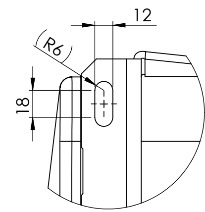
SLOT DETAIL A (TYP) SCALE 2 : 5
