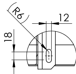
SLOT DETAIL A (TYP) 1:5
